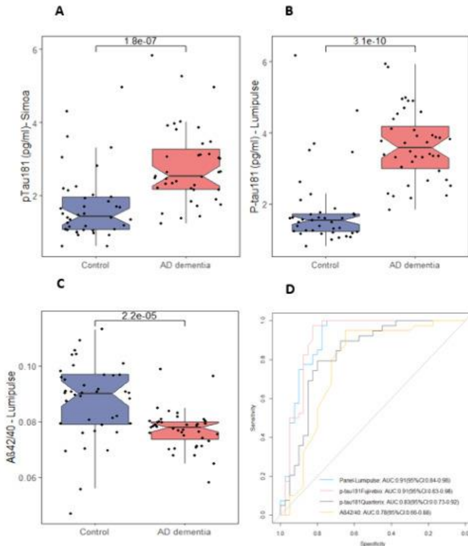
Figure 3. A-C) Boxplots to demonstrate pTau levels and Aβ42/40 measured in 40 AD dementia and 40 control samples. P-values for group differences were calculated using the non-parametric Mann-Whitney U Test. The pTau levels were higher in patients with AD-dementia compared to controls (pTau181 Lumipulse : 2.3-fold; pTau181 Simoa : 1.8-fold). D) ROC curves of the discrimination between controls and AD dementia for the pTau181 and β-Amyloid assays. The pTau181 Lumipulse demonstrated higher accuracy in identifying AD (AUC=0.91, 95%CI:0.83-0.98) than pTau181 Simoa (AUC=0.83, 95%CI:0.74-0.92; DeLong's p=0.004). Similarly, Aβ42/40 Lumipulse achieved an AUC of 0.78 (95%CI:0.66-0.89) (figure 3). Both pTau181 Lumipulse and Aβ42/40 Lumipulse contributed to the diagnostic accuracy of a logistic regression model. However, the resultant AUC remained similar (AUC=0.91, 95%CI:0.84-0.98). We applied logistic regression with Wald's backward selection to assess a panel-Lumipulse. The correlation coefficient \rho is calculated using Spearman's rank correlation analysis. P-tau: phosphorylated tau, AD: Alzheimer's Disease, SD: standard deviation. Group comparisons using the assays were significant, with p-values below 0.05.
