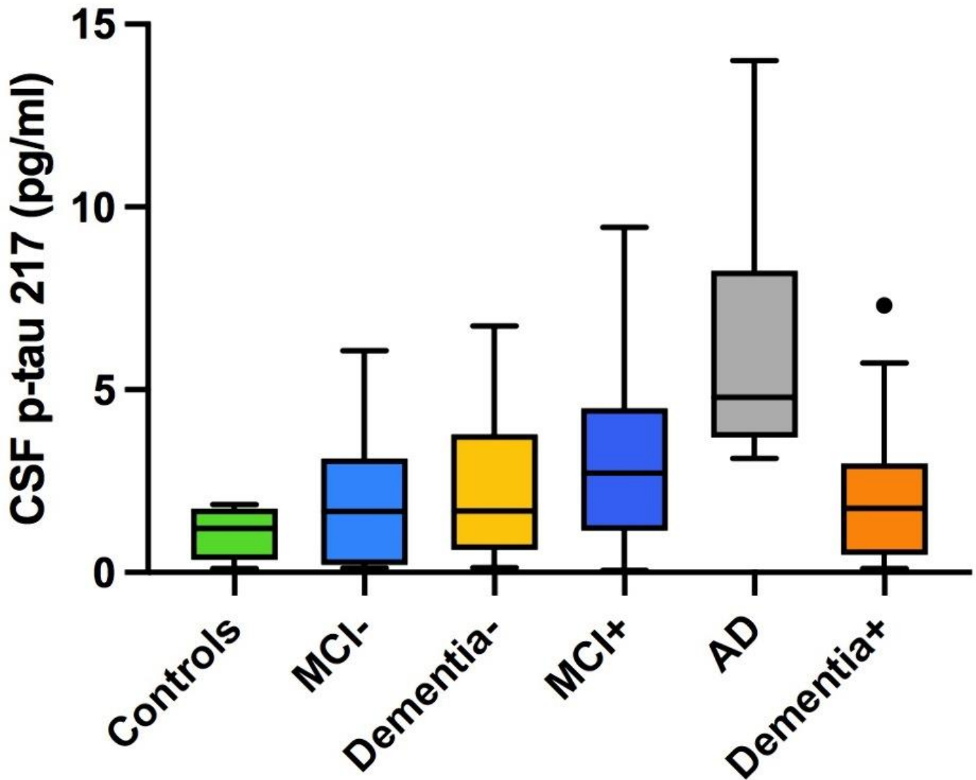
Figure 1: Concentration of CSF p-Tau 217 in CSF in the mixed memory clinic cohort.
