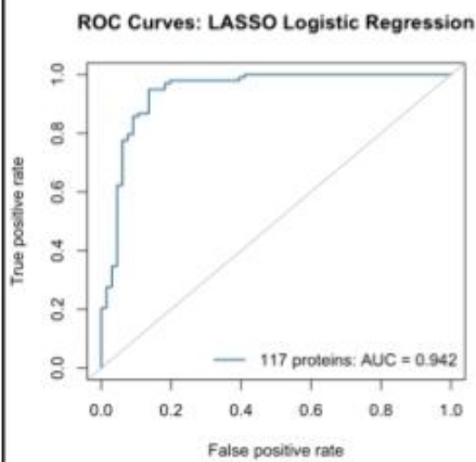
(c) The ROC curves for idiopathic PD prediction.
