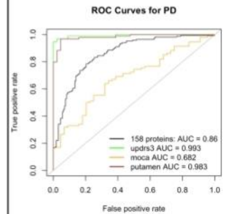
(e) The ROC curves for PD prediction with clinical data.
