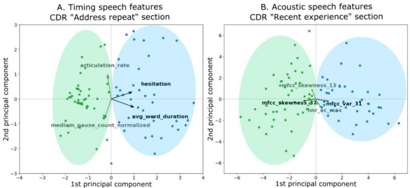
Figure 1. Cluster analysis based on the first two principal components of the speech feature categories. The arrows represent the loadings corresponding to the two most relevant variables contributing to the components (first component: black; second component: grey).
