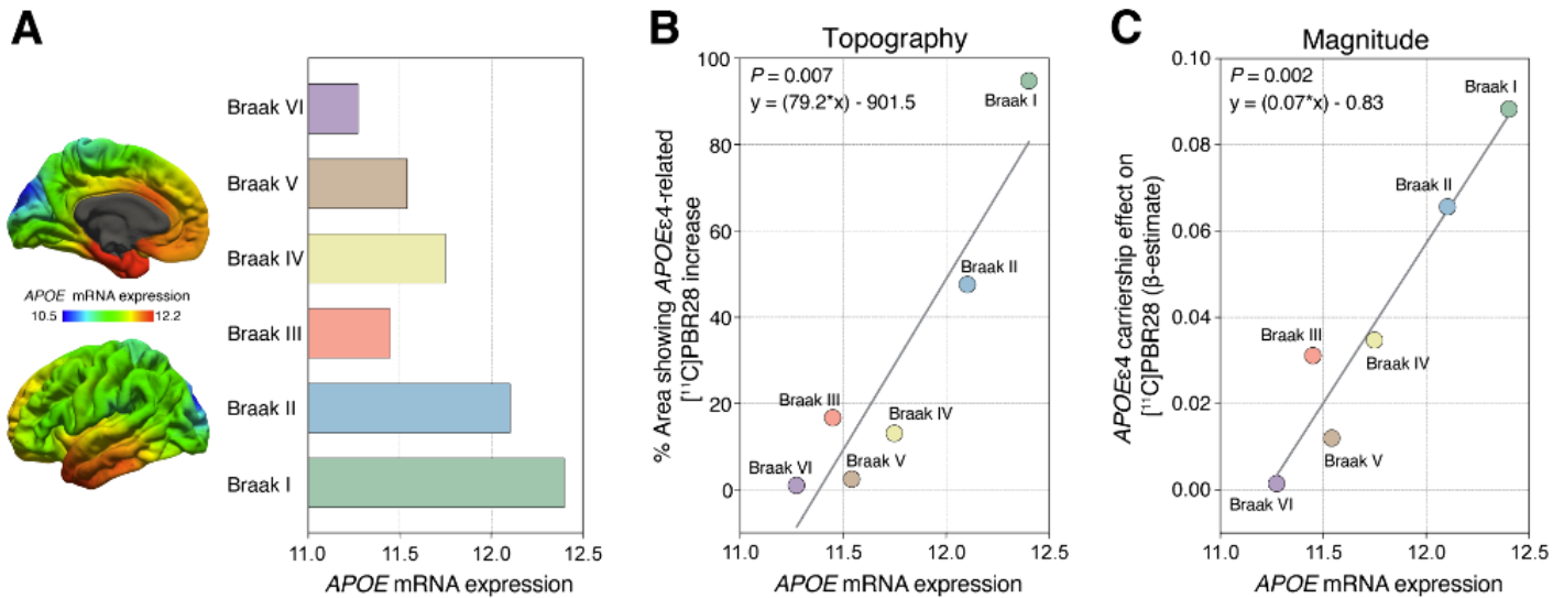
Fig. 3. The brain levels of APOE gene expression predict APOE ε4-related [11C]PBR28 SUVR increase. (A) Brain map of the topographical distribution of APOE mRNA expression in 6 CU individuals obtained from the Allen Human Brain Atlas (left). Average intensity values of APOE mRNA expression in each Braak region (right). (B) Regression analysis testing whether Allen APOE gene expression patterns predict the percentage of the area showing APOE ε4-related [11C]PBR28 SUVR increase across Braak regions in our population. (C) Regression analysis testing whether the Allen brain APOE gene expression patterns predict the magnitude/strength of the association between APOE ε4 and [11C]PBR28 uptake across Braak regions in our population.
